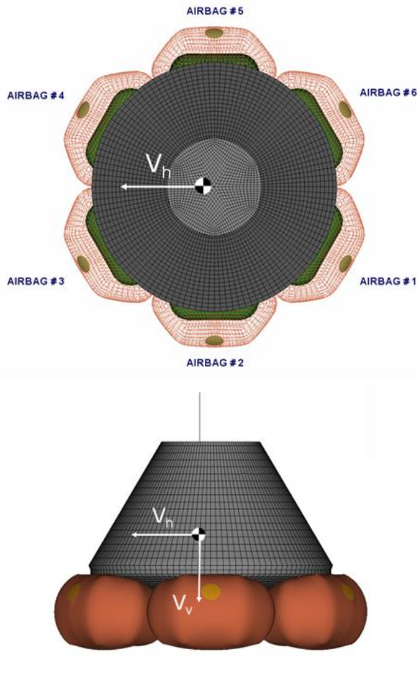
Figure 6: Gen 2 Airbag Numbering and System Definition
